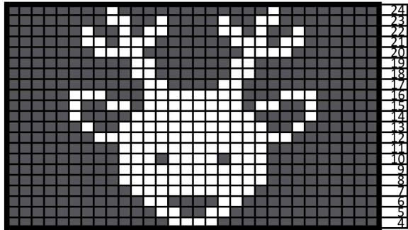
Deer Chart
